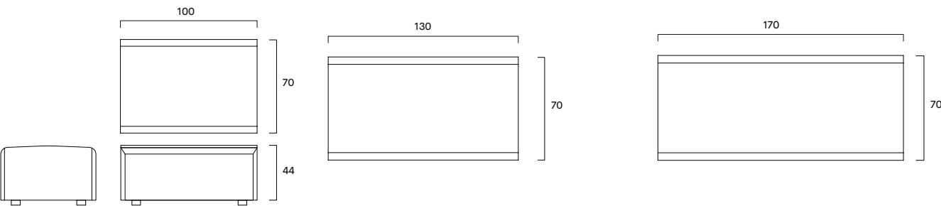
Hug Seat 100 SD54800
