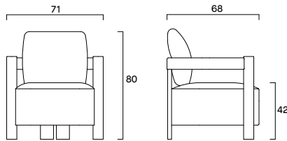
Cloti Lounge FG55700 / 55720
